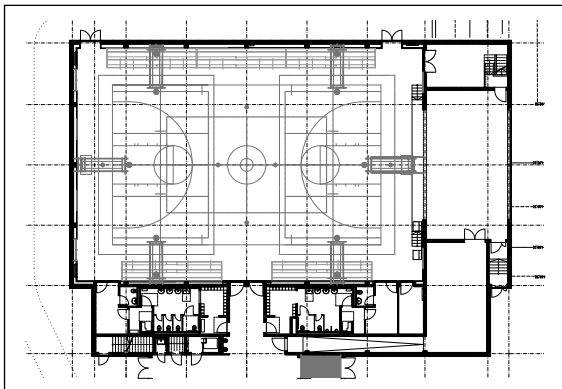
Grundriss Middle School Turnhalle
